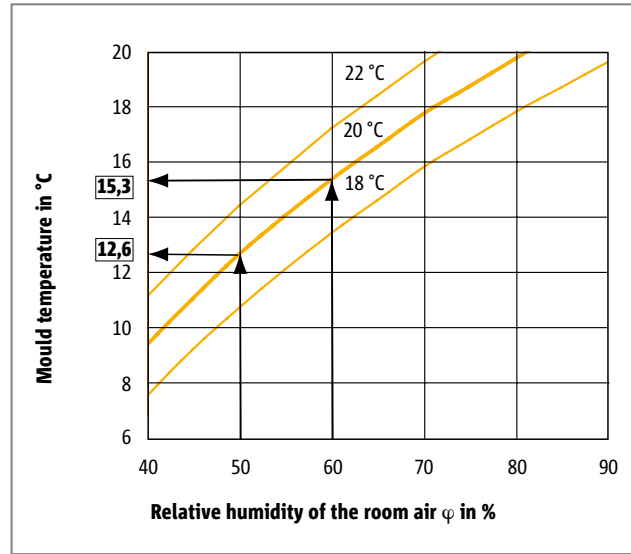
Figure 32: Dependency of the mould temperature on the room air humidity and temperature.
