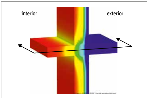
Figure 8a: Illustration of a linear thermal bridge on a linear balcony connection. The left side shows the warm interior with a red surface, while the cold exterior is shown in blue on the right. As the yellow and green spots in the interior corners show, the surface temperatures can drop quite significantly in these areas.
