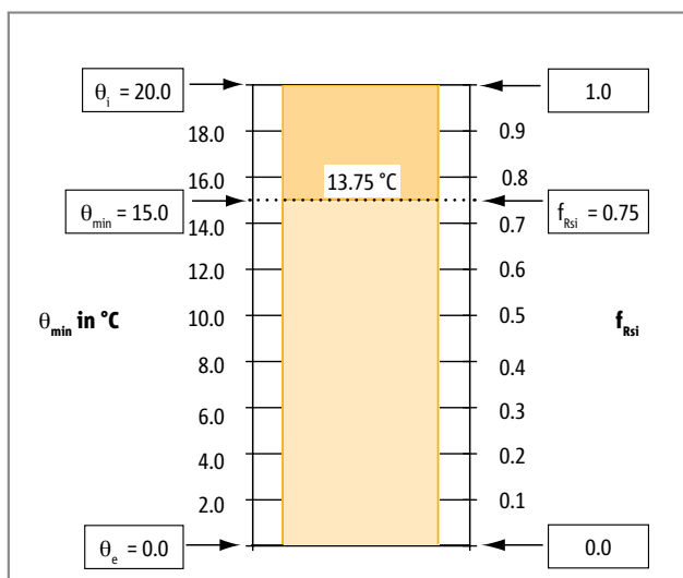
Figure 33: Definition of the f_{Rsi} value.
