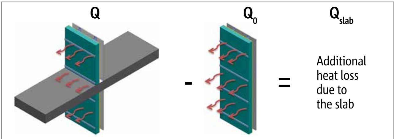
Figure 29: Example of process of determining the linear transmittance of a slab penetrating a wall.
