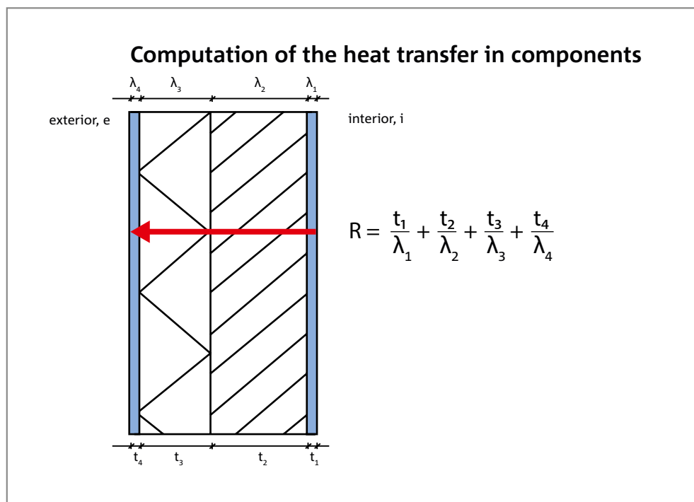
Figure 26: A representation of a wall construction, to define the R value by the thickness of the layers and the corresponding \lambda value.
