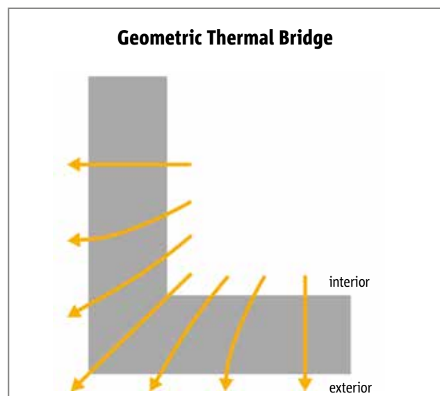
Figure 4: Cross-section of a building corner. The lines show the direction of heat flow from the warm to the cold area. The linear heat flow from an undisturbed wall is affected significantly by the geometric conditions.
