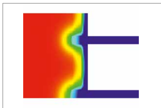
Figure 9b: Top view; this shows a cross-section through the balcony slab presented in 9a. You can clearly see that the heat loss is caused by the two continuous beams. The heat loss is also localised, meaning it is limited to specific spots.
