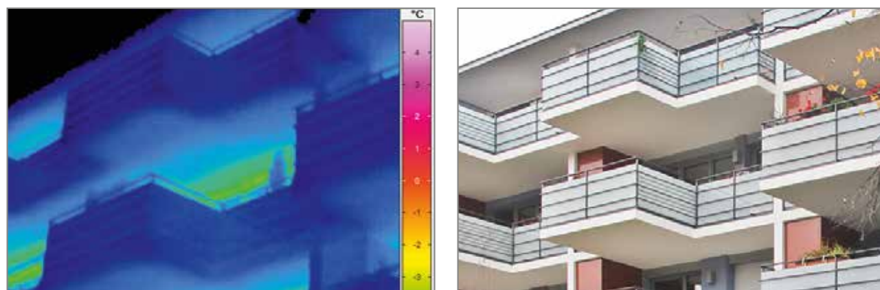
Figure 2: Thermal image of a residential building with minimized thermal bridges and an even temperature distribution along the envelope.
