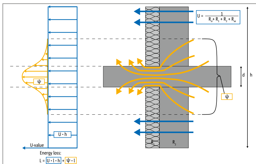
Figure 28: Pattern of heat flow through a building envelope with materials that allow lateral heat flow to a thermal bridge.
