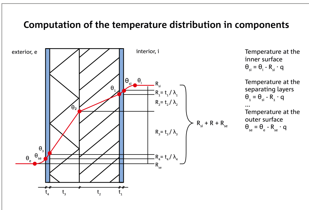
Figure 27: Representation of a temperature profile through a wall. The slope of the temperature profile is defined by the thickness of the layers and the corresponding R value. At the surfaces the surface resistances R_{si} and R_{se} also take effect. On the right hand side you can see how the temperature profile between the different layers is calculated.
