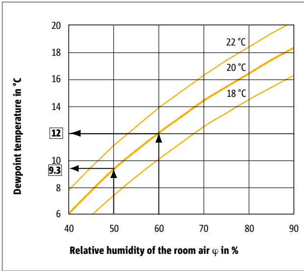
Figure 31: Dependency of the dewpoint temperature on the room air humidity and temperature.
