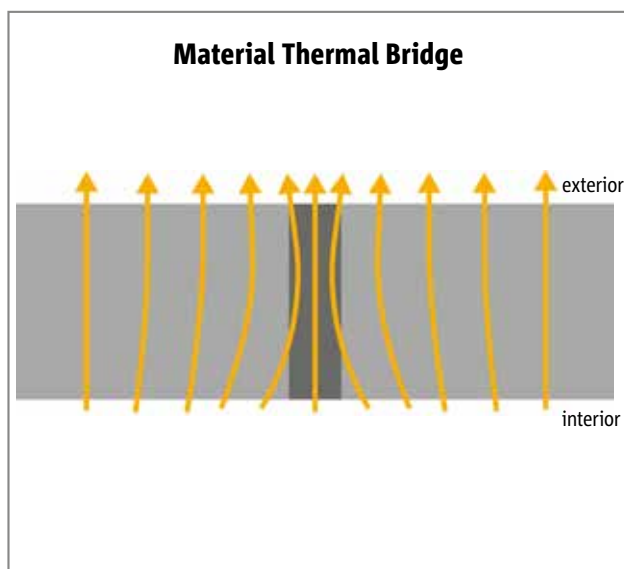
Figure 3: Cross-section through two materials, shows dark grey with high conductivity (steel) and grey with medium conductivity (concrete). The direction of heat flow is shown by the arrows. The heat flows from the warm room (bottom edge of the image) to the colder area (top edge of the image) through the material.
