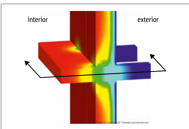
Figure 9a: Illustration of a local thermal bridge on a point balcony connection. In this case, steel beams are connected to a concrete floor from the outside. The left side shows the warm interior with a red surface, while the cold exterior is shown in blue on the right. As the yellow and green spots in the interior corners show, the surface temperatures can drop quite significantly.
