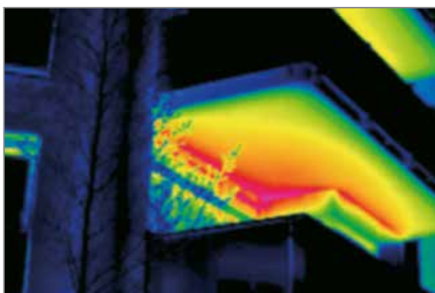
Figure 5: Infrared scan of a balcony thermal bridge with higher temperatures at the exterior slab.
