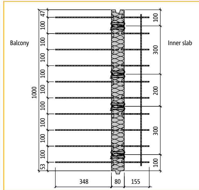
Plan view: Schöck Isokorb® type Q50
