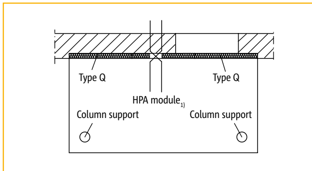
Figure 1: Balcony with column support
