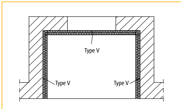
Figure 1: Balcony supported on three sides
