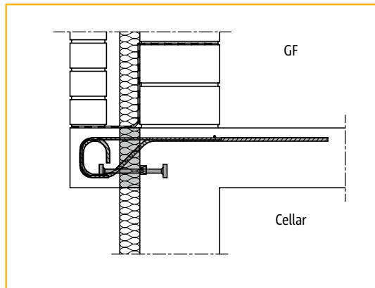
Cross-section between clinker mounting and cellar wall
