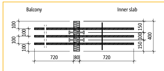
Plan view: Schöck Isokorb® type QP70+QP70
