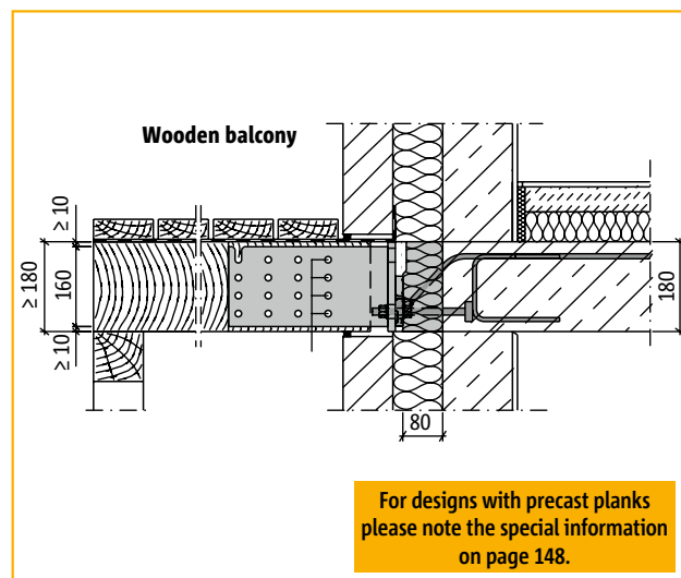
Connection with Schöck Isokorb® type QSH for thermal separation of wooden members from a reinforced concrete inner slab. For more information please contact our design department under 0845 241 3390.
