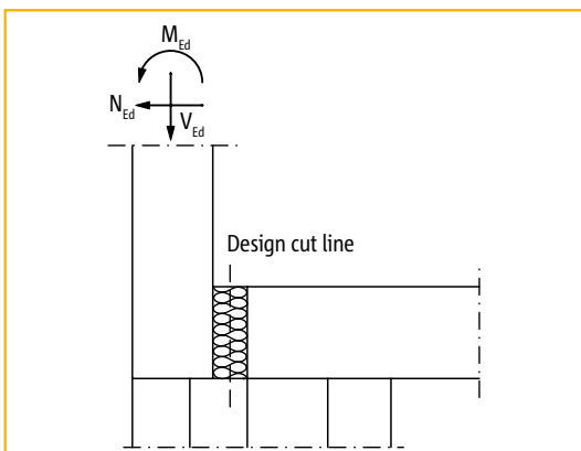
Structural system
