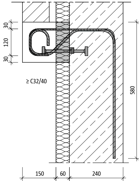
Connection of Schöck Isokorb® type O-WU 24 in the wall area without adjacent inner slab - special design
