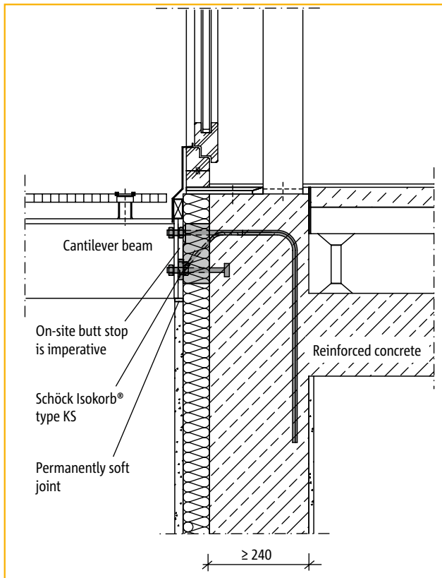
Cleaning balcony to façade
