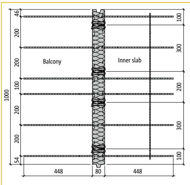
Plan view: Schöck Isokorb® type Q70
