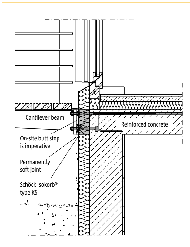
Façade balcony connection
