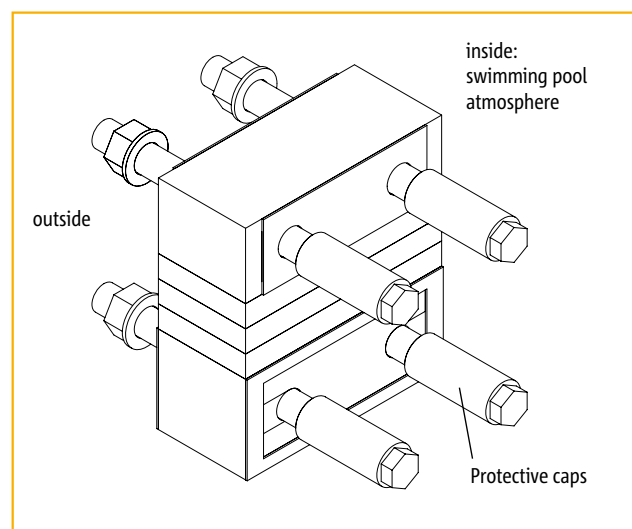
Schöck system-solution for protection in high chlorine environments
