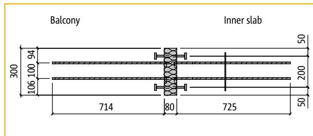
Plan view: Schöck Isokorb® type QP60
