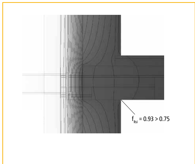
Figure 12b: Isothermals for connection 12a
