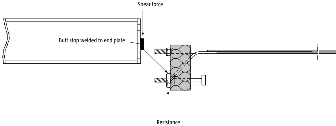
Side view: Imperative butt stop for the connection of steel fin to Schöck Isokorb®
