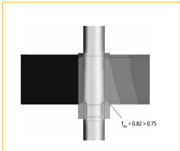
Figure 13b: Isothermals for connection 13a
