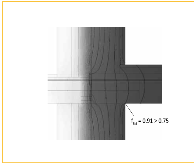
Figure 11b: Isothermals for connection 11a
