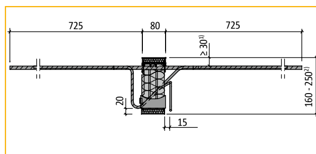
Schöck Isokorb® type K60 to K100
