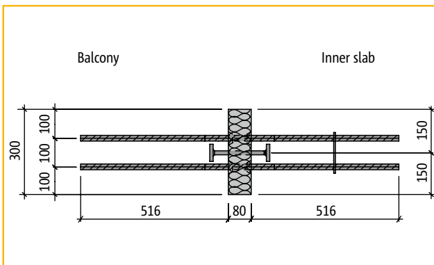
Plan view: Schöck Isokorb® type QP40+QP40
